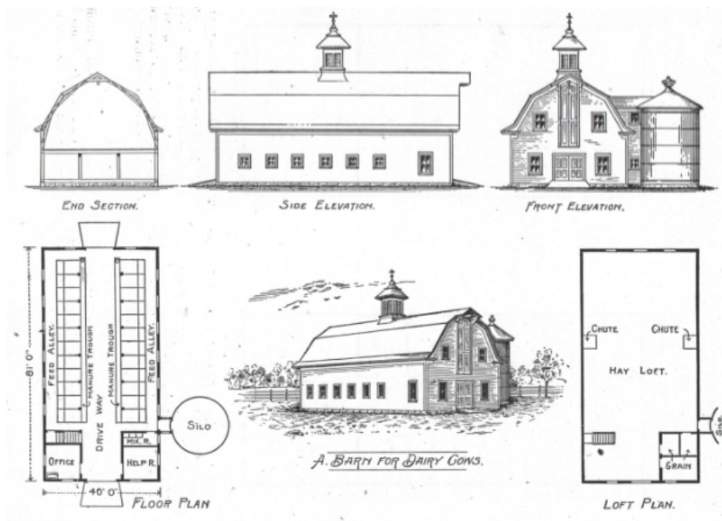
Example of dairy barn plan from Radford's Practical Barn Plans , 1907
